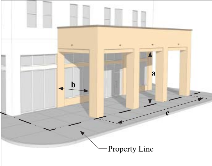
FIGURE 5.3. GALLERY DIMENSIONS
